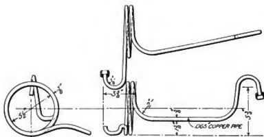
Figs. 3157-3158. Steam Gage Pressure Pipe. Atlantic (4-4-2) Locomotive, P. R. R.
